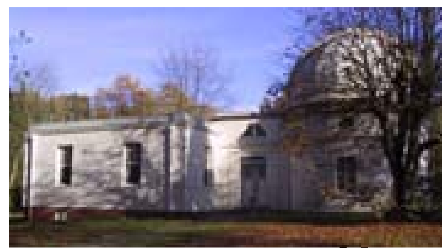
Lippert-Astrograph
