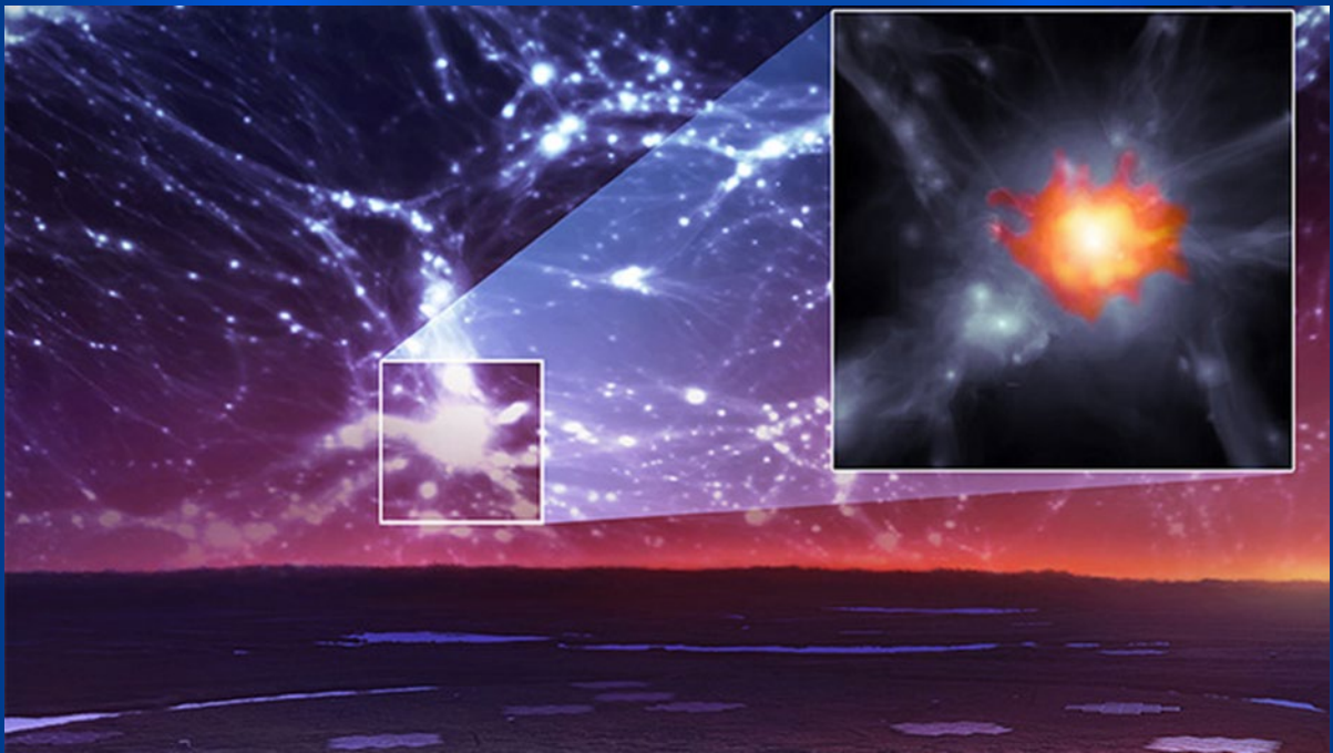
Simulation (credit: Marcus Brüggen)
